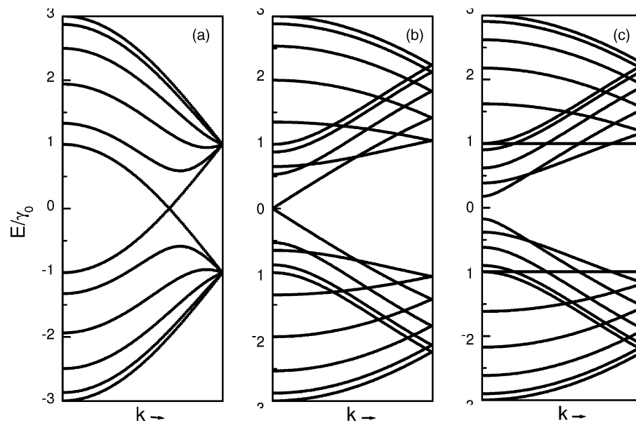
Fig. 11. Electronic band structure of nanotubes (a) (5, 5) , (b) (9, 0) and (c) (10, 0) derived by zone-folding of the band structure of the graphene sheet; a is the nearest-neighbor C–C separation and \gamma_0 = 2.9 eV.
