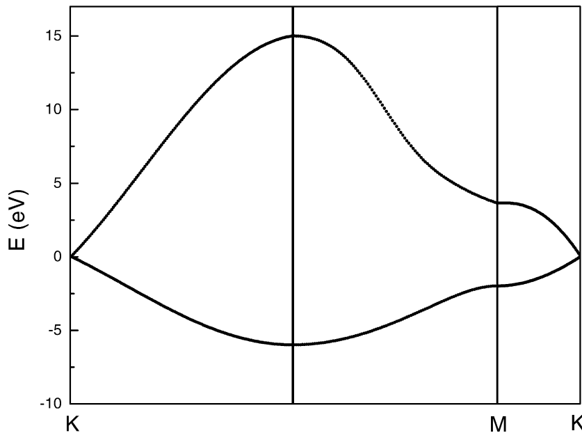
Fig. 10. The electronic band structure of a graphite sheet calculated within a \pi -band tight-binding model. The valence \pi and conduction \pi^* bands show degeneracy at the \mathbf{K} points in the Brillouin zone at the Fermi level.
