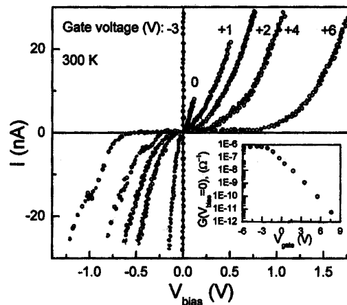
Fig. 27. The I – V characteristics of a nanotube FET for various values of the gate voltage V_g (after [68]). A negative V_g leads to ohmic behavior while a positive V_g results in a strong suppression of the current at low bias voltage V and non-linear I – V curves at higher bias.
